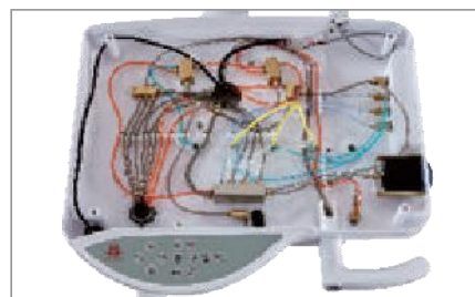
Neat piping assembly of the table 整洁的进口管道工具盘装配
